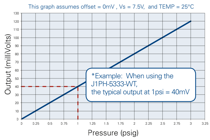
Typical Transfer Function (Sensor pn J1PH-5333-WT): Vout = (40 * P) + Offset ± Error
